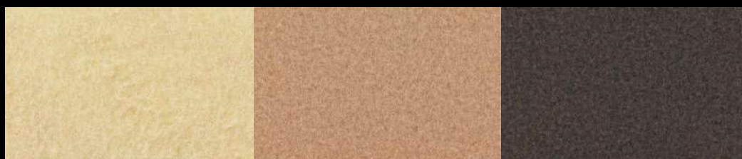
9506 Ivory
